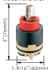
Cartridge (Type F) Model : 892-6159
