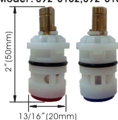
Cartridge (Type I) Model : 892-6162, 892-6163
