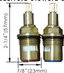
Cartridge (Type J) Model : 892-6164/892-6165
